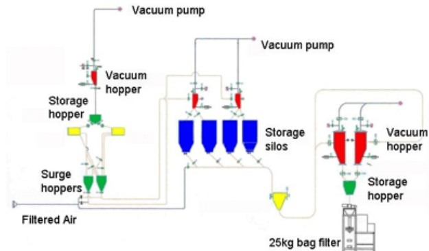
A Typical Example of a dense phase vacuum conveying system.
